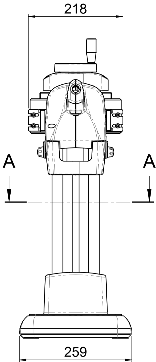
FRONT VIEW
